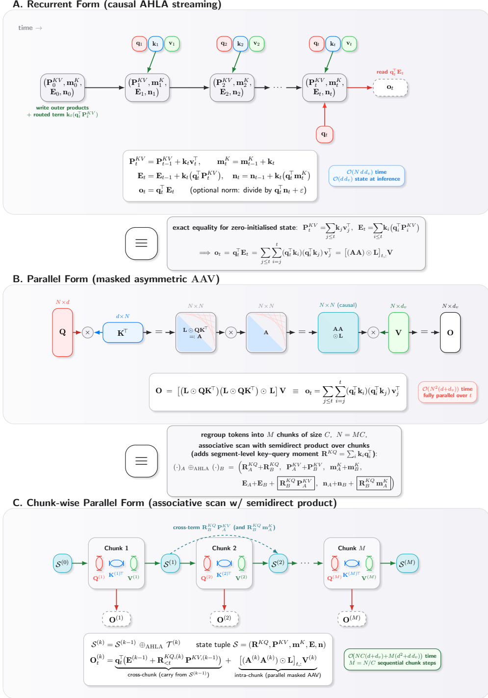
Figure 2 Three equivalent views of Asymmetric Higher-order Linear Attention (AHLA). (A) The recurrent form maintains a constant-size state tuple \mathcal{S}_t = (\mathbf{P}_t^{KV}, \mathbf{m}_t^K, \mathbf{E}_t, \mathbf{n}_t) . (B) The parallel form materializes the asymmetric causal weight (\mathbf{AA}) \odot \mathbf{L} with \mathbf{A} = \mathbf{L} \odot \mathbf{QK}^T and applies it to \mathbf{V} . (C) The chunk-wise parallel form interpolates between (A) and (B) via an associative scan over the augmented tuple \mathcal{S} = (\mathbf{R}^{KQ}, \mathbf{P}^{KV}, \mathbf{m}^K, \mathbf{E}, \mathbf{n}) .
