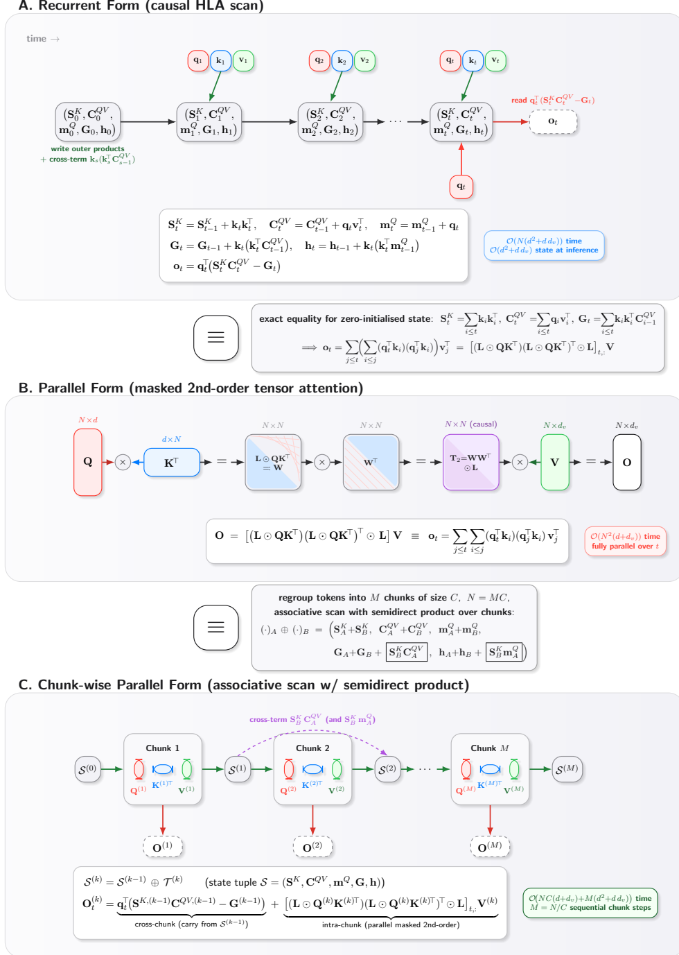
Figure 1 Three equivalent views of Higher-order Linear Attention (HLA, second order). (A) The recurrent form maintains a constant-size state tuple \mathcal{S}_t = (\mathbf{S}_t^K, \mathbf{C}_t^{QV}, \mathbf{m}_t^Q, \mathbf{G}_t, \mathbf{h}_t) , with two additional cross-summaries \mathbf{G}_t, \mathbf{h}_t that enforce strict causality at second order. (C) The chunk-wise parallel form interpolates between (A) and (B): the sequence is split into M chunks of size C , intra-chunk computation evaluates the masked second-order form in parallel.
